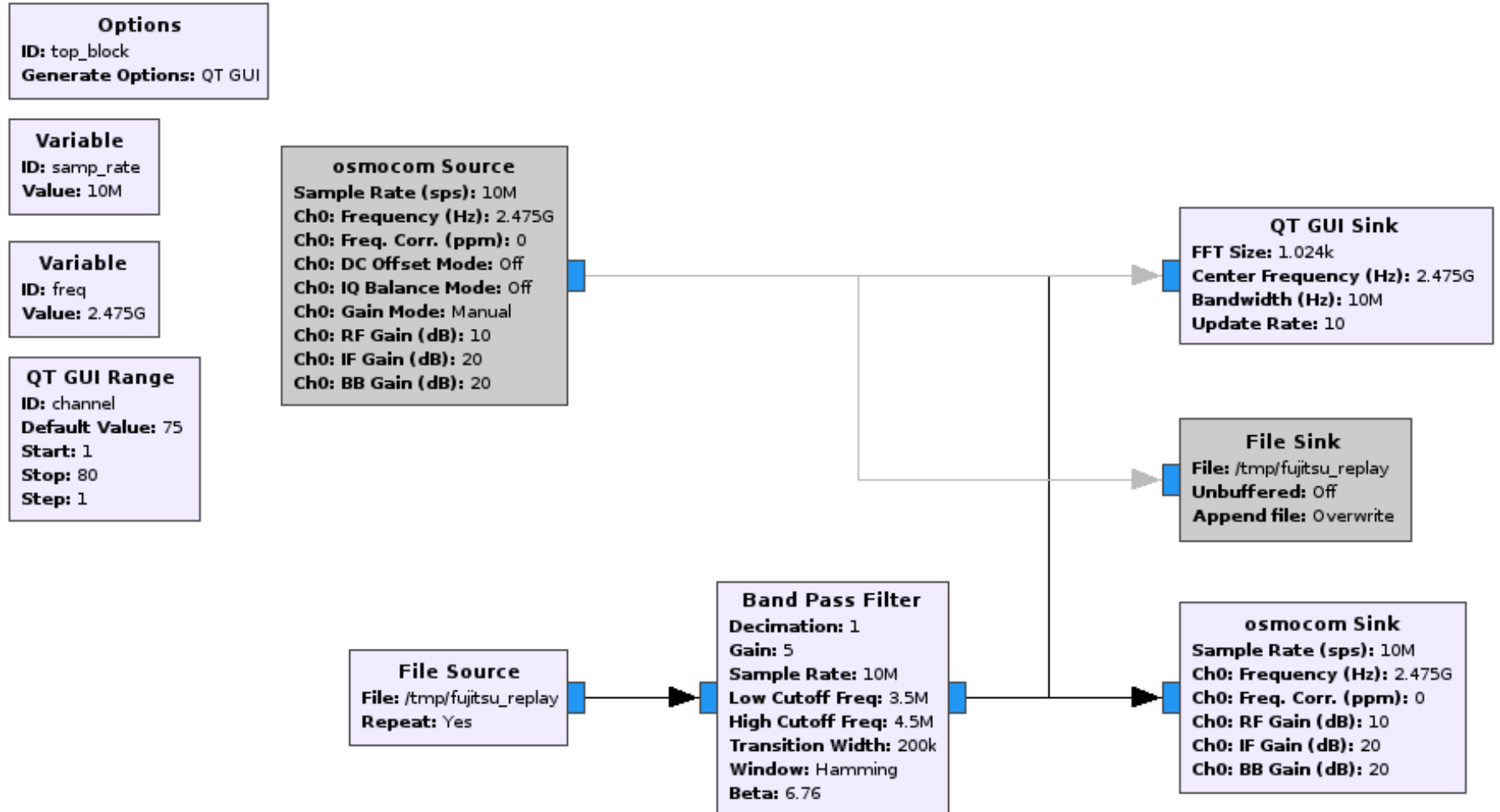
Simple GNU Radio Companion flow graph for replay attacks using a software-defined radio (HackRF One)
